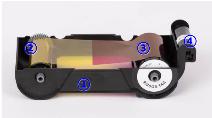
Figure 6 Ribbon cartridge features
