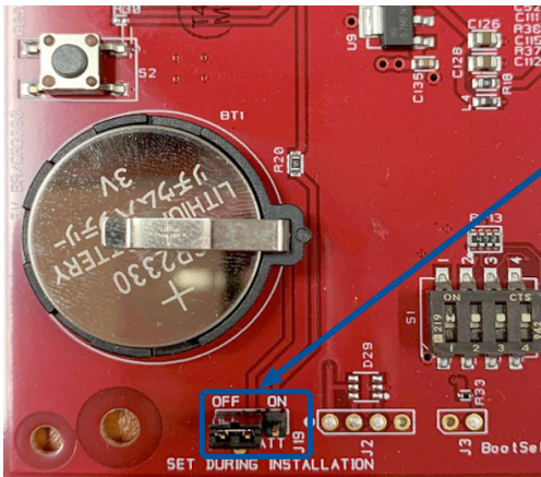
LP2500 with the jumper in the OFF position.
