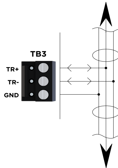
Port 2 to serial I/O devices
