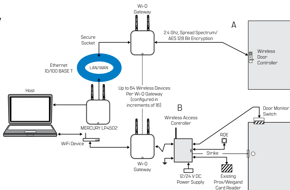
Figure 2 Hardware Overview
