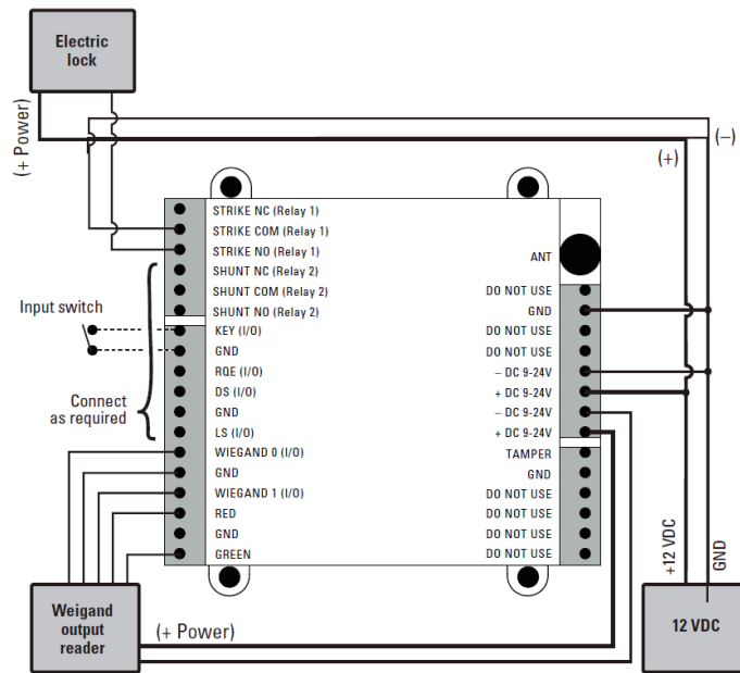
Figure 13 Connecting Devices to a WAC
