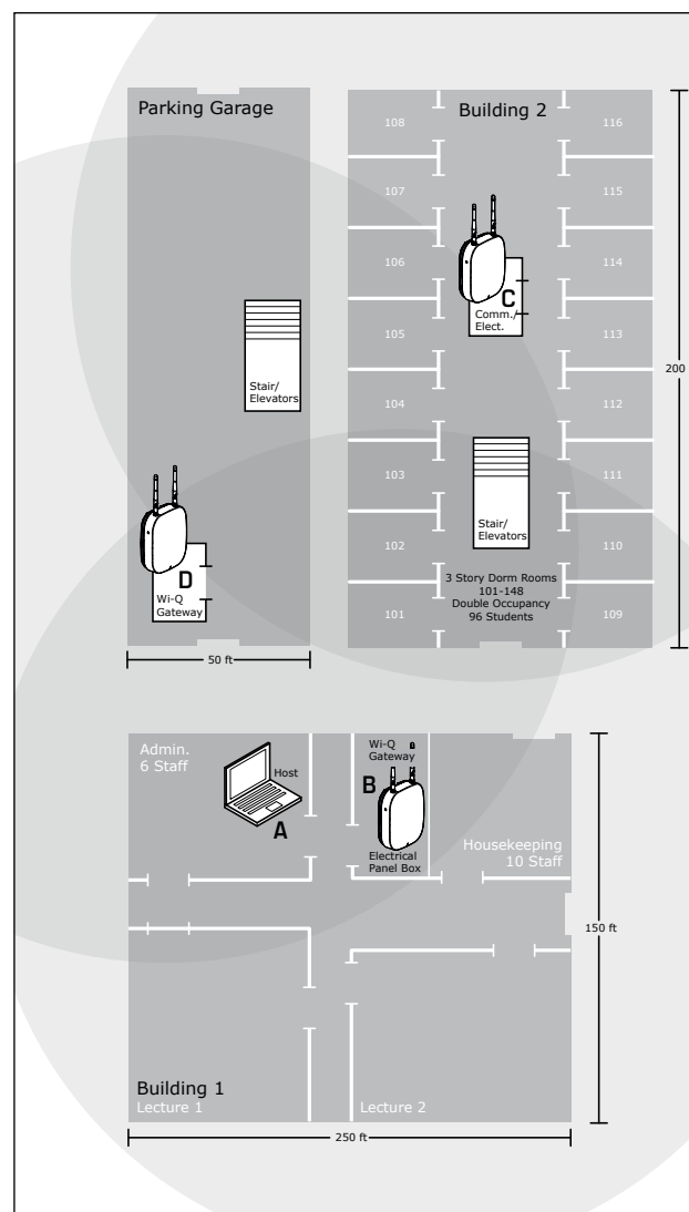
Figure 4 Sample Site Installation Plan
