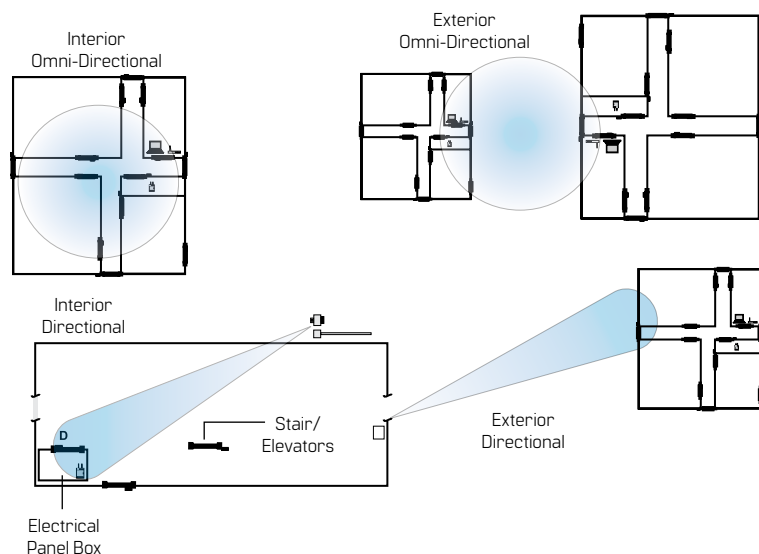
Figure 5: Selecting the Antenna Type That Best Suits the Installation
